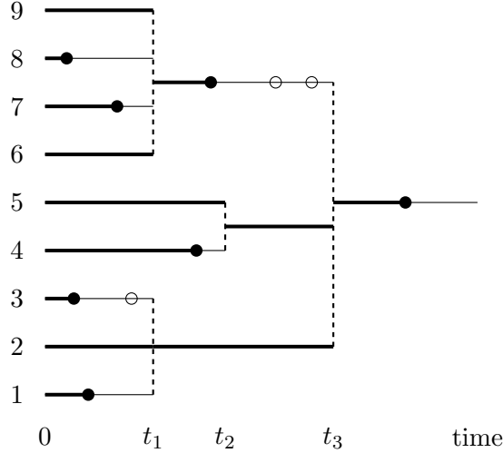
Figure 1: A realization with n = 9 particles labeled by \{1, \dots, 9\} , and coalescent events occurring at times t_1, t_2 and t_3 . Open branches are indicated as thicker lines, and any mutation that falls onto an open (resp. closed) line is depicted as filled (resp. unfilled) circle.
